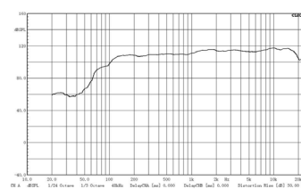
Frequency Response
