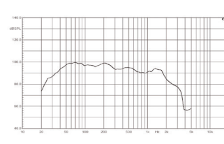
Frequency Response
