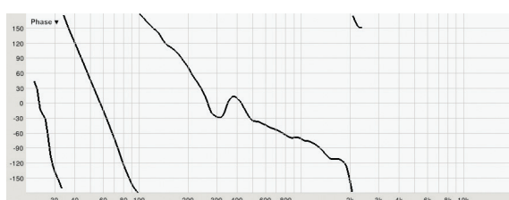
Phase
